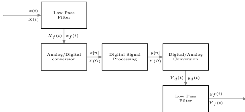
Figure 1 The path of signal in digital processing.
